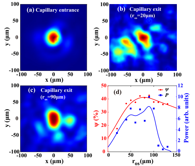
FIG. 2. Laser guiding at 3 \times 10^{15}\text{ W/cm}^2 in the curved plasma channel. (a) Beam spot at the capillary entrance. (b) and (c) Beam spots at the capillary exit for r_{\text{os}} = 20 and r_{\text{os}} = 90\text{ }\mu\text{m} , respectively. (d) Dependence of energy concentration ( \Psi ) and transmitted power ( P ) on the offset distance r_{\text{os}} , the fitted smoothing spline curves show their evolution tendency.
